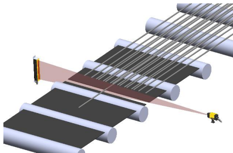
Detection of small bars (hot or cold) on a wide table
